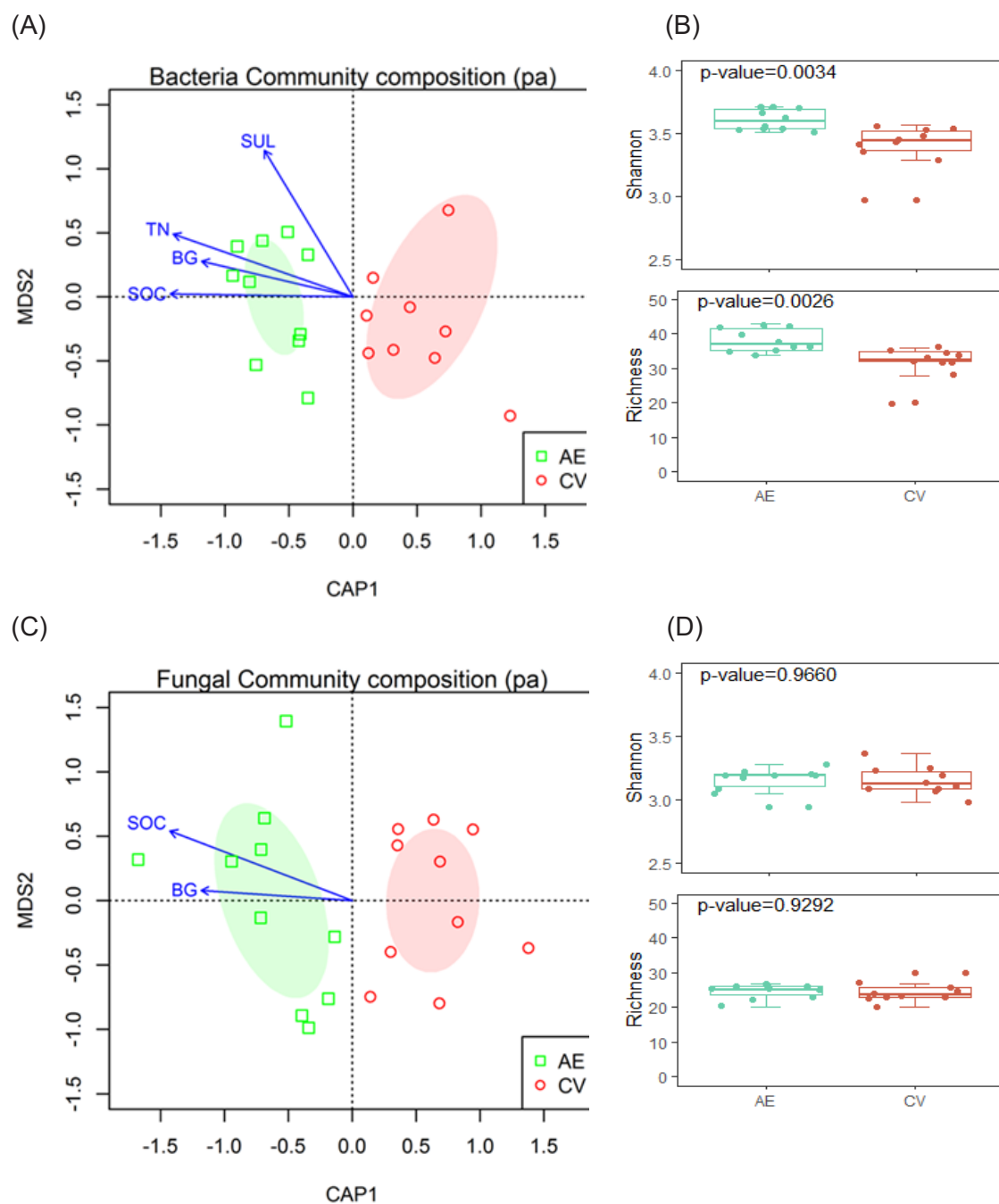
Figura 5: Changes in the bacterial and fungal community between agroecological (AE) and conventional management (CV). A and C: Constrained Analysis of Principal Coordinates (CAP) analysis of the community beta diversity of bacterial and fungal communities based on Altgower distance. The significance of differences between microbial communities was identified using permutational multivariate analysis of variance (PERMANOVA). Vectors represent significant correlations between ordination and soil properties: SOC (soil organic matter), SUL (sulfatase), TN (total N), BG ( \beta -Glucosidase). Ellipses indicate one unit of standard deviation from the centroid of each group. B and D: Community alpha diversity of the bacterial and fungal communities. Microbial abundance was determined based on the presence-absence matrix generated from the 16S and ITS1 rRNA amplicons after DGGE analysis, with significant differences at P < 0.05 and P < 0.01 , respectively (MLM).
