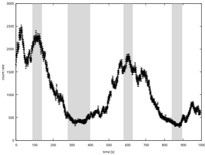
Figure 12. The spectra extracted around maxima and minima (shaded areas) of the first exposure done on July 20 are shown on the right. The spectra traced in blue are extracted from the minima shaded on the light curve shown on the left, the red from the maxima. The count rate has been normalized to the level of the second maximum, by multiplying the first maximum spectrum (red stars) by 0.7, and the minima respectively by 3.2 (first minimum, x-es), and by 2.7 (second minimum, squares).
