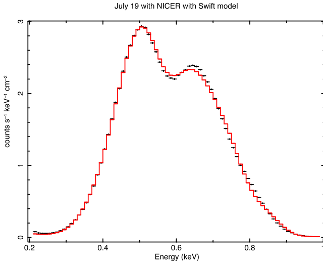
Figure 13. The spectrum of V1674 Her on the left, plotted as a function of energy, was measured on July 19. The LETG spectrum plotted on the right with the natural units of wavelength of the grating was also measured on the same day, although at a different time. The best fit with the blackbody+edges model of Drake et al. (2021) is shown in both panels. The fit is not perfect for the NICER spectrum, and since in the LETG, we are able to resolve the absorption and emission lines; it is clear that this one-component fit is not adequate.
