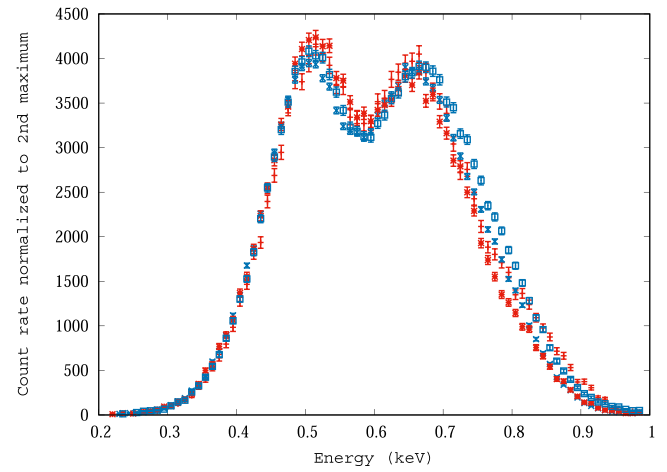
Figure 12. The spectra extracted around maxima and minima (shaded areas) of the first exposure done on July 20 are shown on the right. The spectra traced in blue are extracted from the minima shaded on the light curve shown on the left, the red from the maxima. The count rate has been normalized to the level of the second maximum, by multiplying the first maximum spectrum (red stars) by 0.7, and the minima respectively by 3.2 (first minimum, x-es), and by 2.7 (second minimum, squares).
