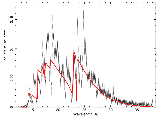
Figure 13. The spectrum of V1674 Her on the left, plotted as a function of energy, was measured on July 19. The LETG spectrum plotted on the right with the natural units of wavelength of the grating was also measured on the same day, although at a different time. The best fit with the blackbody+edges model of Drake et al. (2021) is shown in both panels. The fit is not perfect for the NICER spectrum, and since in the LETG, we are able to resolve the absorption and emission lines; it is clear that this one-component fit is not adequate.
