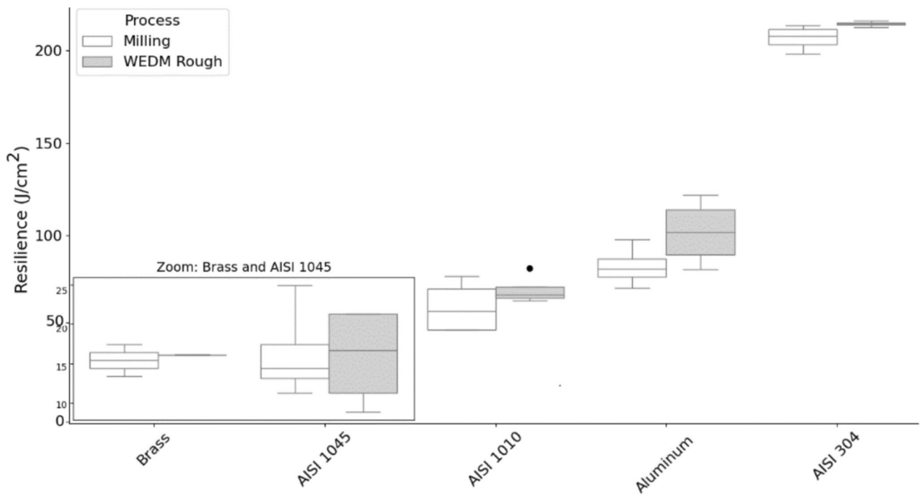
Fig. 3 Material resilience in Charpy tests
