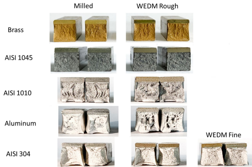
Fig. 4 Fracture analysis of specimens made from different materials with notches created by milling and WEDM, tested in Charpy impact tests; transverse section view
